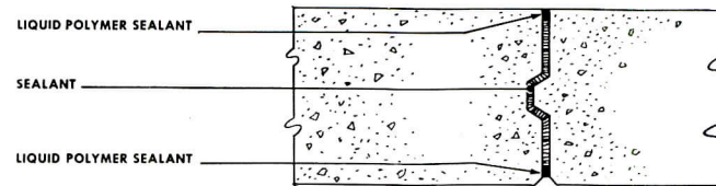
Expansion Joint in Concrete Wall
