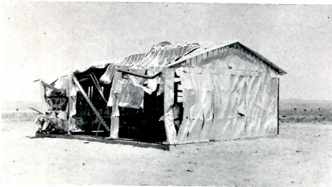
STEEL — Rigid-frame building; 3.1 psi overpressure
