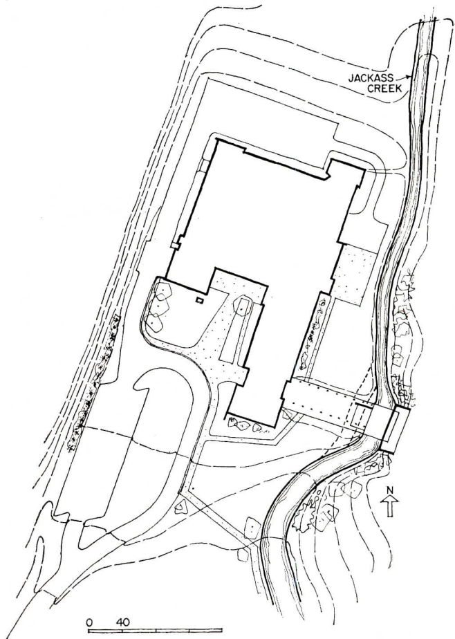
PLOT PLAN
