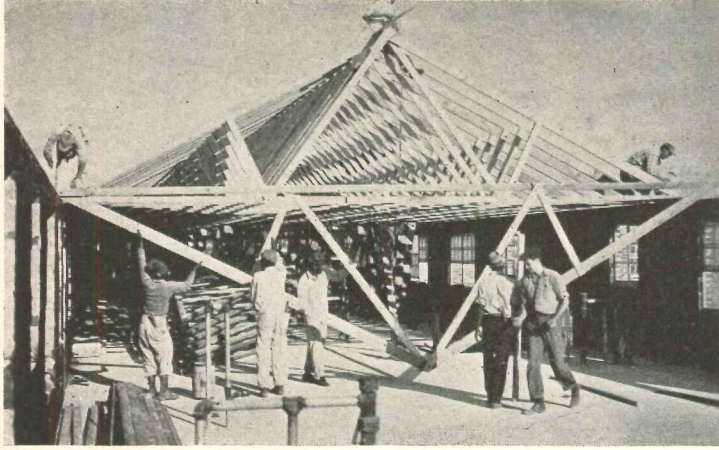
"Timber Design and Construction Handbook" illustrates (above) design procedures and details of timber assemblies and structures based on experience
