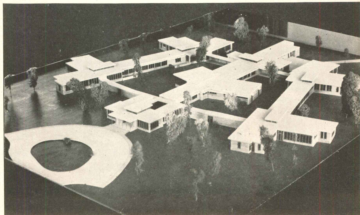
Central axis contains common areas for all patients; outer wings are four separated nursing units, each with three patient classifications
