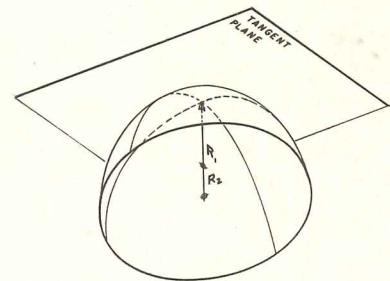
Surface of Positive Curvature
