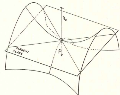
Surface of Negative Curvature
