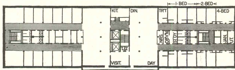
SECOND, THIRD FLOOR PLAN
