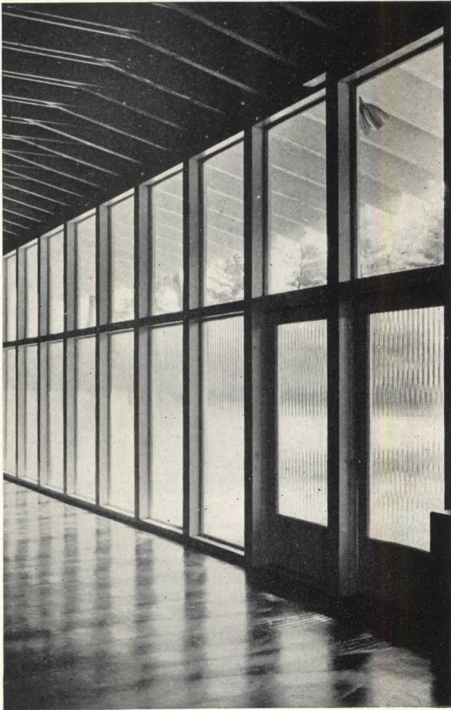
Lower window sections in the auditorium (left and above) are fitted with translucent glass to obscure view of simultaneous outside activities; clear glass upper sections give view of trees and sky. Exposed ceiling beams are painted a dark terra cotta, and extend to form sunshade over south windows. Roof is surfaced with white marble chips
