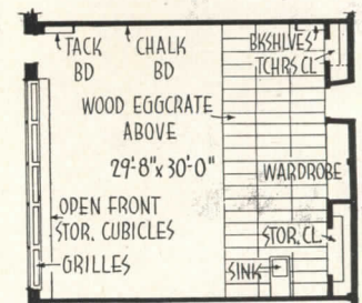
TYPICAL INTERMEDIATE CLASSROOM
