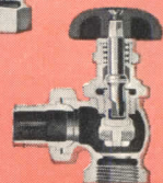
SARCO Radiator Valve No. 1141
