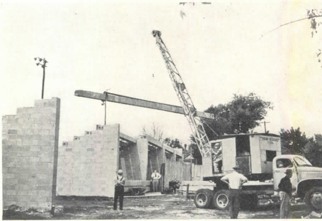
31-ft beams span between conventional concrete block piers
