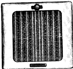
Model WJ-13 Bilt-in-Wall Small-Room Heater. 110 volts A.C.; 1320 watts; 4507 BTU. Approximate wall opening required: 9½" x 11½".
