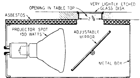
Reflected Downlighting
