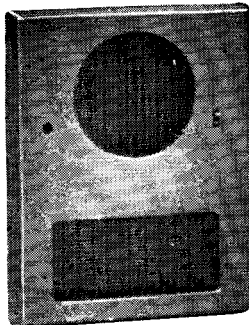
Model WJ-13 Bilt-in-Wall Small-Room Heater. 110 volts A.C.; 1320 watts; 4507 BTU. Approximate wall opening required: 9½" x 11½".
