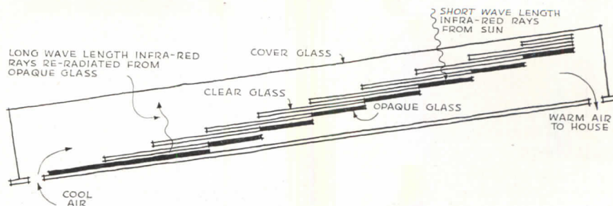
Heat trap developed at University of Colorado. Short waves pass through the clear glass and heat the opaque, re-radiating long waves to which clear glass is not transparent
