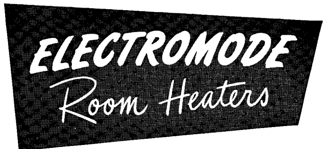
Model W-12 Bilt-in-Wall Room Heater. 230 volts A.C.; 1500 to 3000 watts; 5122 to 10245 BTU. Approximate wall opening required: 14¼" x 18¼".
