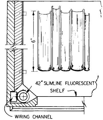
Bookcase Lighting
