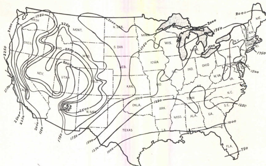
Approximate number of sunny hours during heating season. Dark days in the North are offset by longer season — days when normal mean temperature is 65° F. or below
