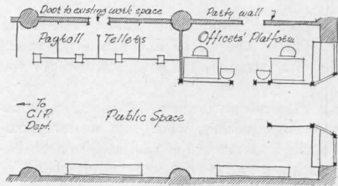
into quiet dead-end. Payroll window situated at corner permits longer lineups. Work space is moved downstairs with directors' room, rest rooms, and vaults
