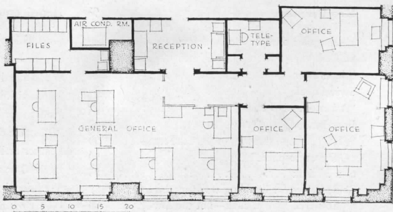
General office is dimensioned to give best daylight to each pair of desks, not for the absolute minimum of space. Private offices are adequate, but they are not pretentious
