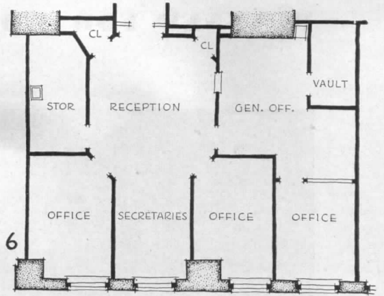
6. A similar office with more emphasis on the reception room. Here the visitors get more attention than either the executives' offices or the office employees. But here too, as in any well-planned office, the files, the stores, the lavatory, the coats, are hidden away in inside space
