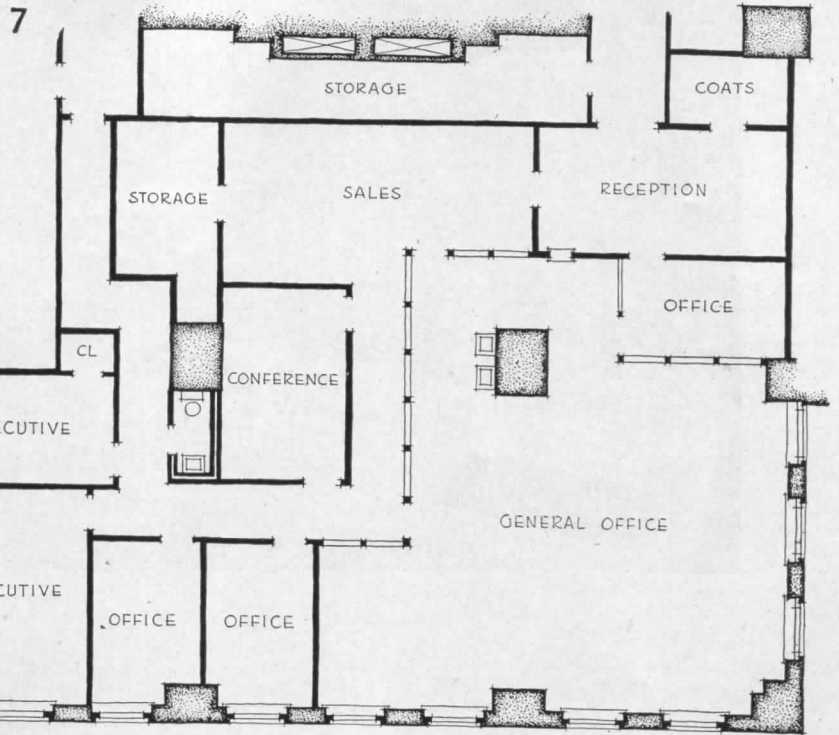
7. In every building there are certain areas where the space is exceptionally deep. Here is a plan which is just about the ultimate in the use of dark space. Salesmen are supposed to be out selling; their desks don't need daylight. But the office workers get good space. Conference room is mechanically ventilated
