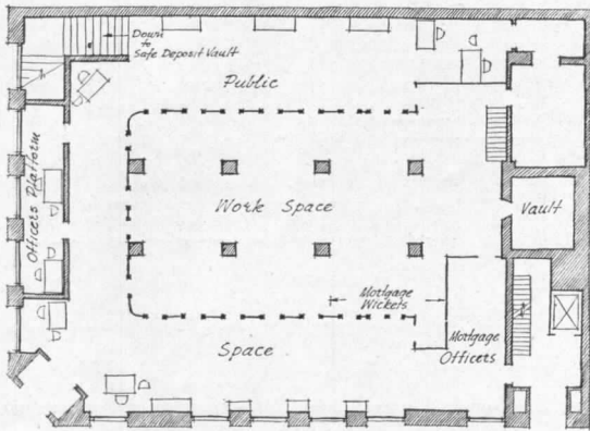
Existing plan
