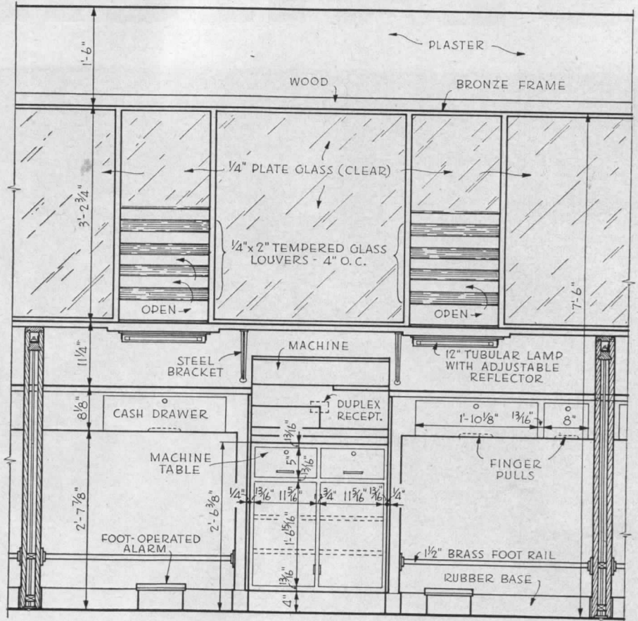
ELEVATION - BACK OF COUNTER SCALE 1/2" = 1'-0"
