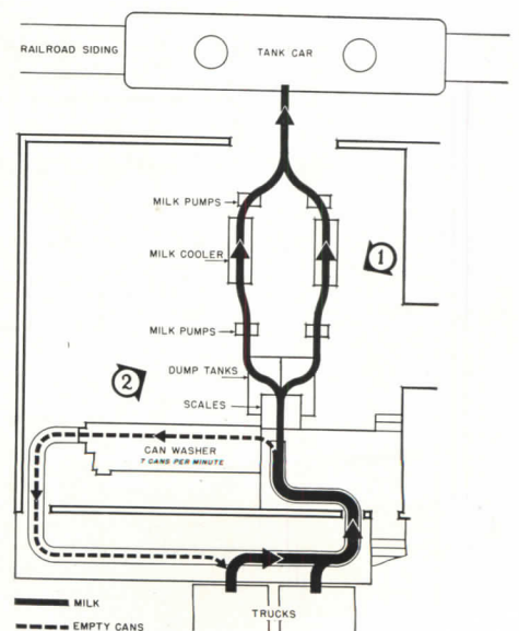
2. The milk is first weighed (at right), then pumped through coolers (center, left), and pumped again through the doors at left into a tank car on the siding.
