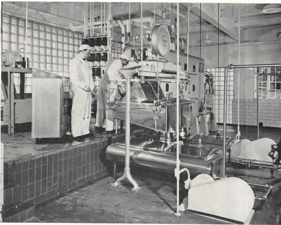
1. On this raised platform, the milk cans enter, are emptied into scales (as shown), washed, sterilized, and returned outside, all within five minutes' time.
