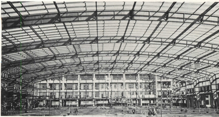
Fig. 9. The "trading floor" of Rotterdam's Corn Exchange, now under construction, will boast the world's largest glass-concrete roof—50,000 sq. ft. and only three inches thick. Here engineer Polivka and architect J. F. Staal had to meet the most rigid requirements in terms of light, sound, and atmospheric control. Precision was guaranteed by prefabricated panels (below) on light steel purlins carried in turn by rigid frames (above).
