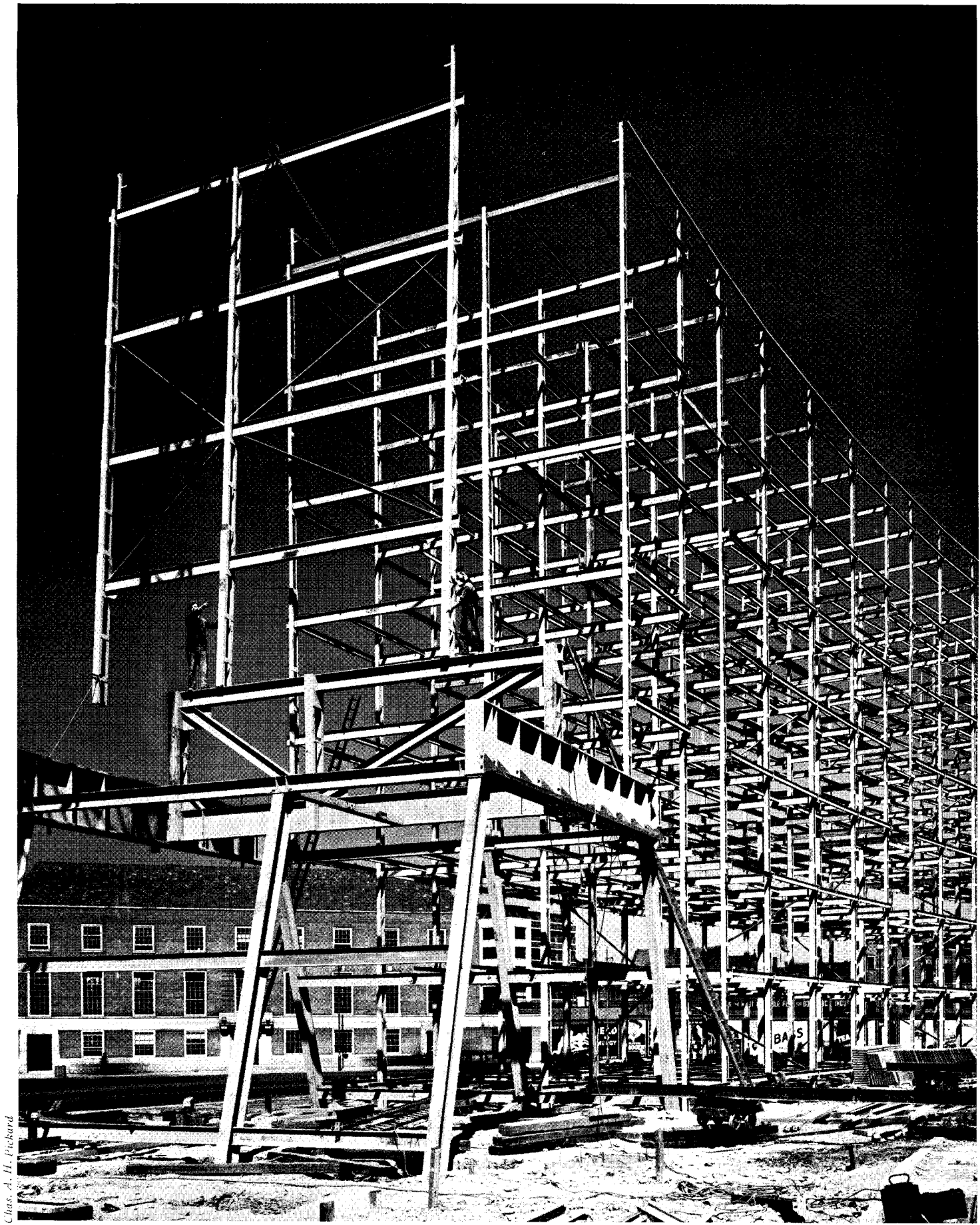
Quarry Hill Flats, under construction at Leeds, England. One of the steel frames being hoisted to position.
