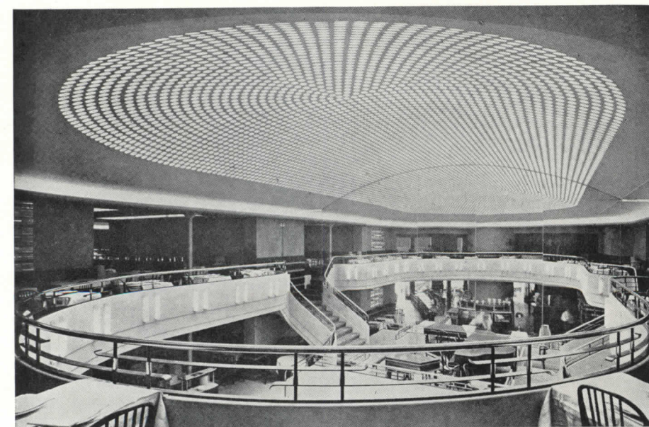
Fig. 8. In this cafe in Paris, architect Roux-Spitz has achieved a thin and shallow translucent dome by means of a system, poured in place and similar to Fig. 1.
