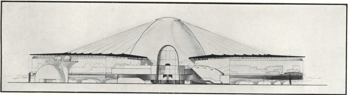
Front elevation
