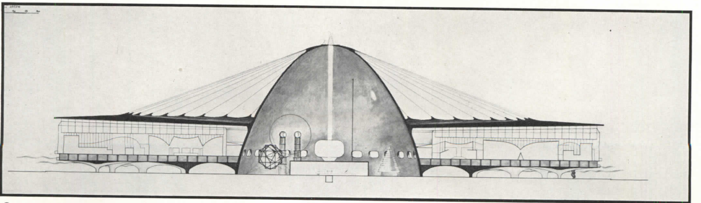
Cross section
