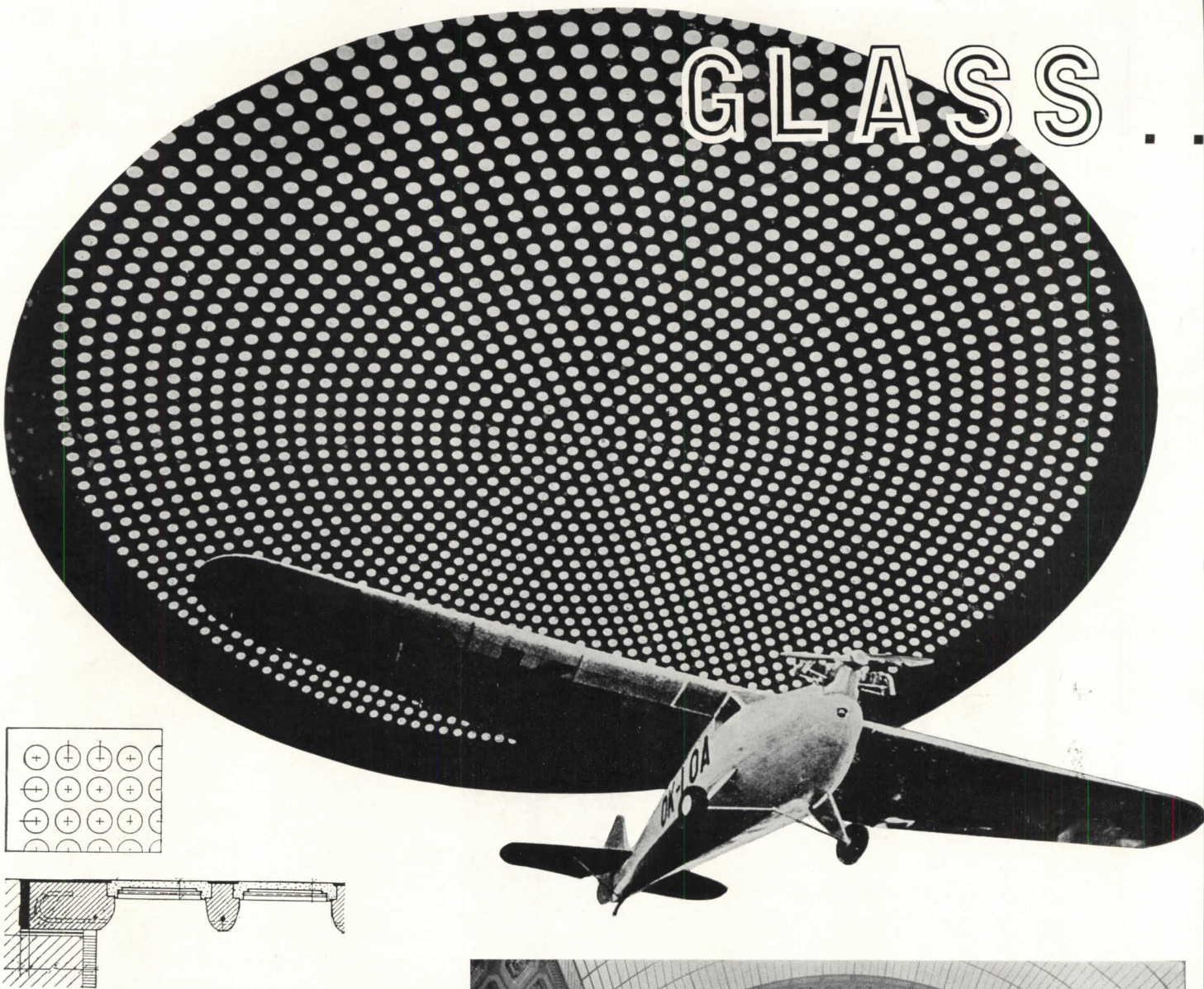
Fig. 1. Interior of Polivka's dome for the Czech Pavilion, Paris, 1937. With a 50-ft. diameter and an over all thickness of only 3 \frac{1}{5} in., this dome was built in place on special forms. Figs. 9 and 10 show similar construction.
