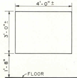
BLACKBOARD SECTIONS
