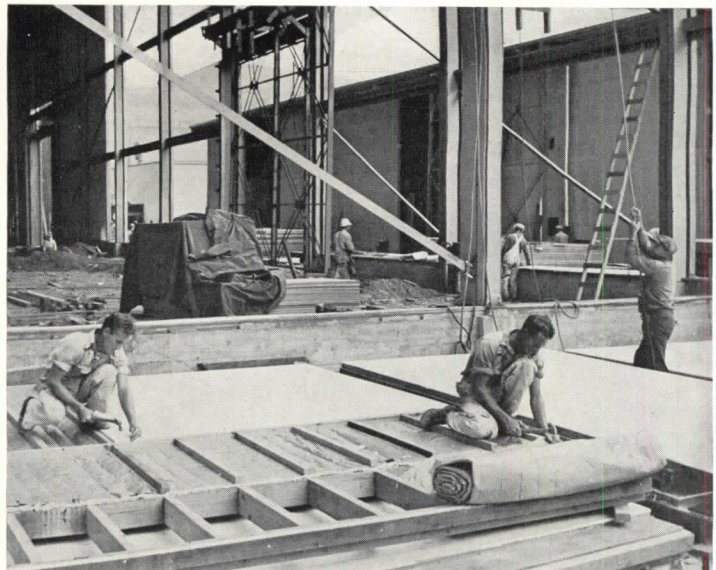
2. Wall panels are prefabricated on the ground. . . .
