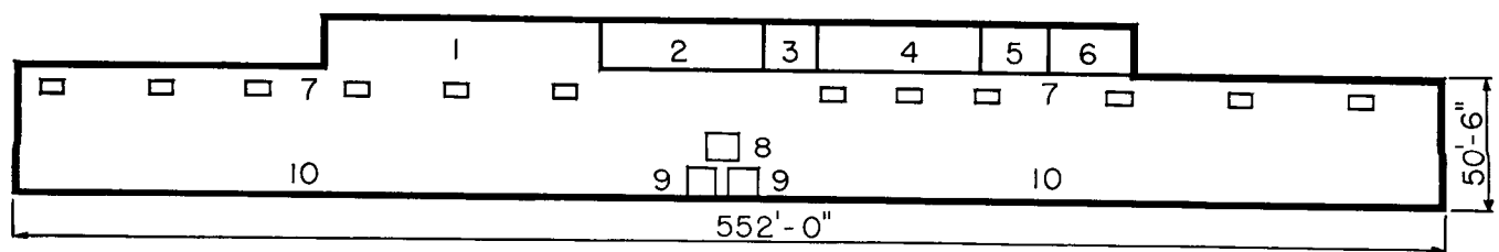
Diagrammatic layout of factory for fabrication of concrete units: 1. Fabrication of reinforcing. 2. Mold repairs, etc., 3. Dynamo, 4. Office, 5. Samples, 6. Mess hall, 7. Vibrating tables, 8. Concrete mixers, 9. Sand and gravel, 10. Drying space.
