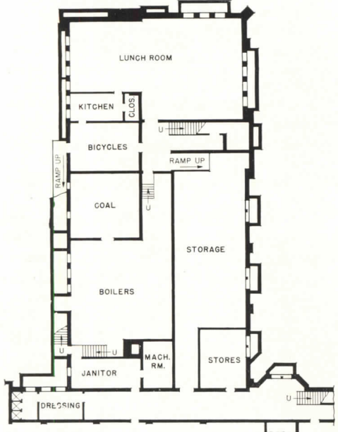
Part of basement
