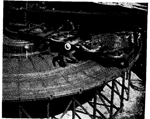
4 Forms in place, reinforcing begins . . . 5 with pre-crimped radial steel; then . . . 6 concentric reinforcing is threaded off.
