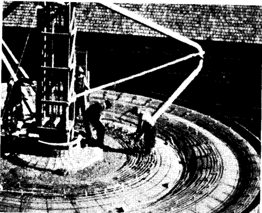
7 Pouring begins; speed is guaranteed by . . . 8 the rotating, rubber hose and . . . 9 rotating screed gets an accurate profile.
