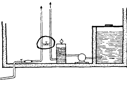
Typical cross-connections resulting in back-siphonage and contamination of potable water. Top: A safe faucet has its outlet at least 1/2 inch above highest possible water level. Similar cases often arise in water closets, particularly those equipped with flush valves which do not leave satisfactory air checks; and in tubs. A direct cross-connection between city water and cistern water, circled in the lower drawing, should be eliminated.
