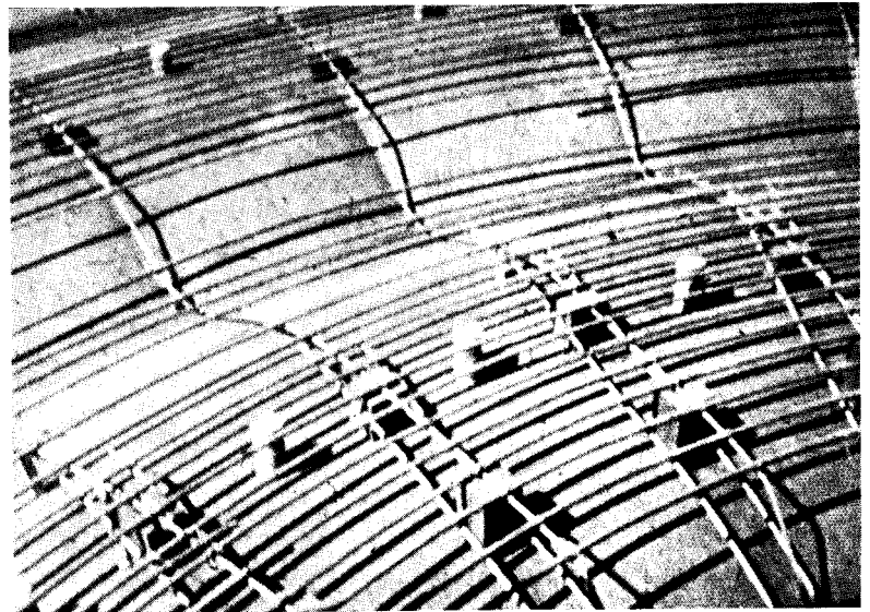
Reinforcing of horizontal plate
