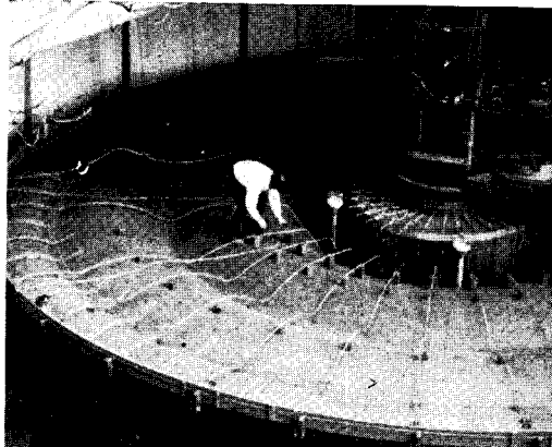
4 Forms in place, reinforcing begins . . . 5 with pre-crimped radial steel; then . . . 6 concentric reinforcing is threaded off.
