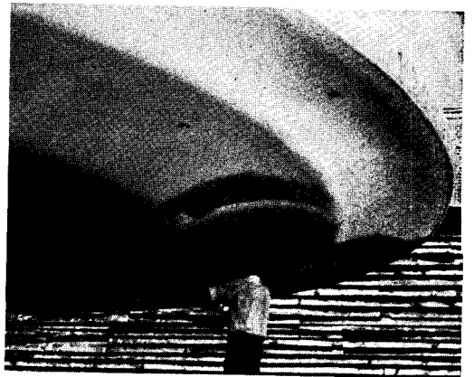
10 Then formwork is removed . . . 11 top surface waterproofed . . . 12 and the underside spray-painted.
