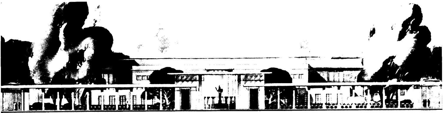
The central ticket office (above) with its flanking shelters will be built, while behind it lie Messrs. Murphy and Wischmeyer's conception of what the administration unit should look like. The concrete shelter has a typical section (right) which varies only as to balustrades, screen walls, etc., and grade; along the sides of the auditorium, its roof and floor levels follow the grade.
