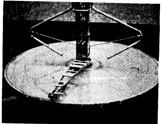
7 Pouring begins; speed is guaranteed by . . . 8 the rotating, rubber hose and . . . 9 rotating screed gets an accurate profile.
