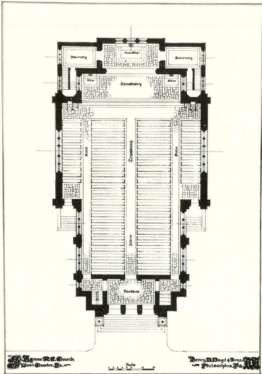
ST. AGNES ROMAN CATHOLIC CHURCH, WEST CHESTER, PENNSYLVANIA Henry Dagit & Sons, Architects
