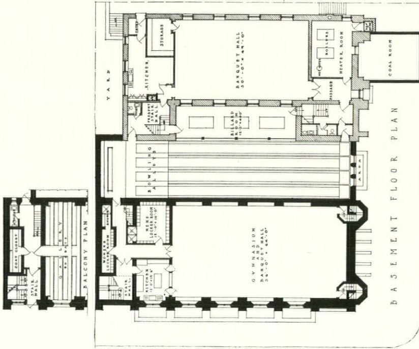
FORT GEORGE PRESBYTERIAN CHURCH 186th Street and St. Nicholas Avenue, New York City Clarence Brazier, Architect
