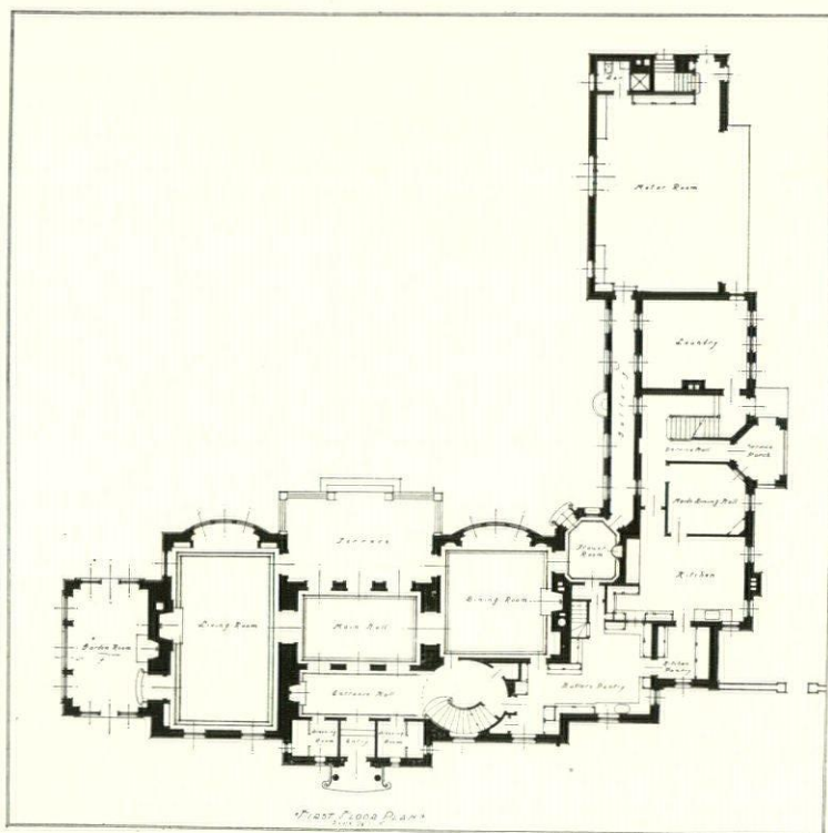
RESIDENCE OF MR. AND MRS. WILLARD M. CLAPP, CLEVELAND HEIGHTS, OHIO Frank B. Meade and James Hamilton, Architects
