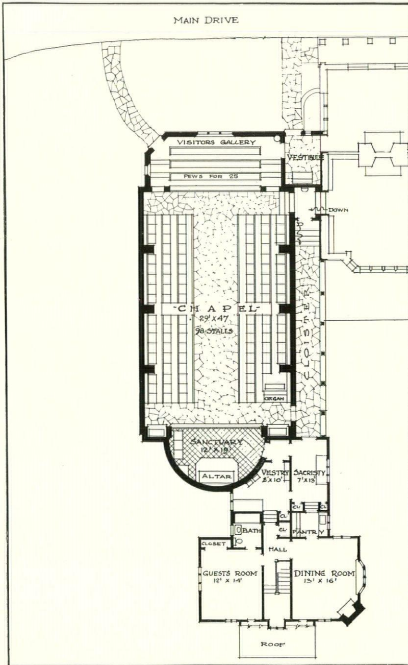
FLOOR PLAN OF THE SACRED HEART CHAPEL, BEACON, N. Y.
