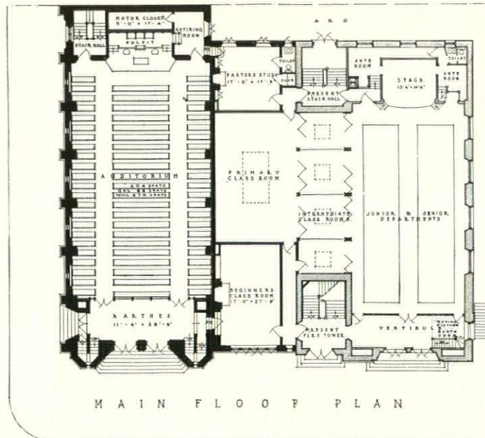
FORT GEORGE PRESBYTERIAN CHURCH 186th Street and St. Nicholas Avenue, New York City Clarence Brazer, Architect
