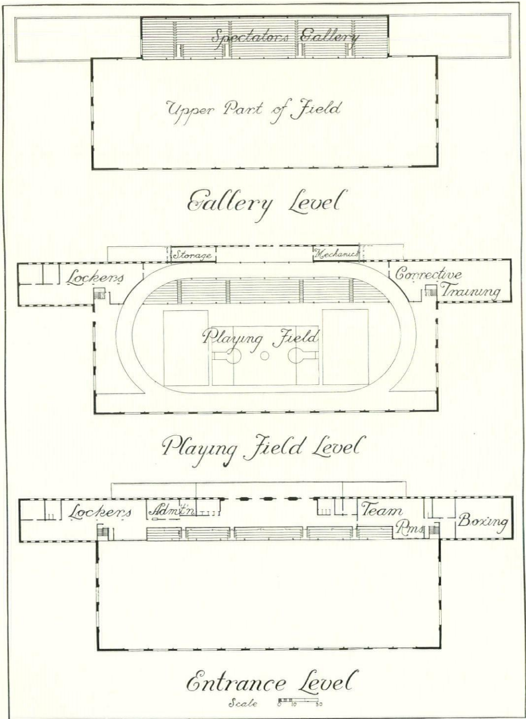
FIELD HOUSE OF THE UNIVERSITY OF WEST VIRGINIA Davis, Dunlap & Barney, Architects
