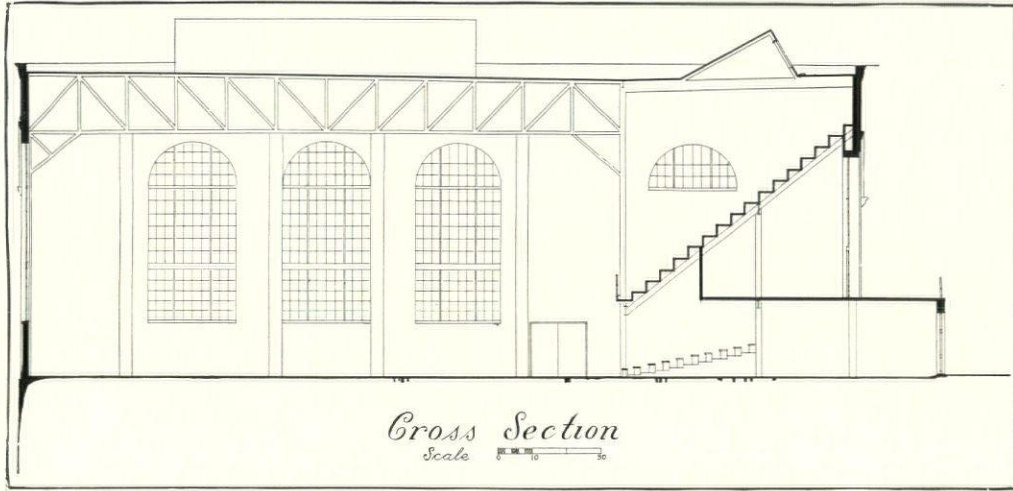
FIELD HOUSE OF THE UNIVERSITY OF WEST VIRGINIA
